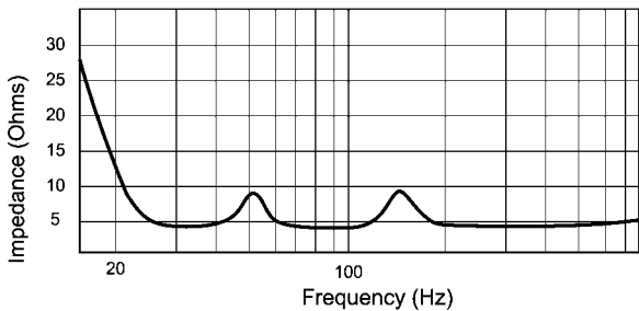
ARS-215 Impedance
